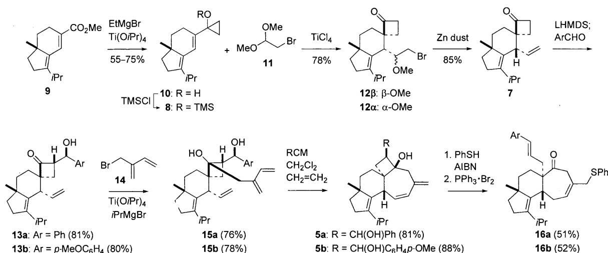
Scheme 2. Construction of the tricyclic core. AIBN = 2,2'-azobisisobutyronitrile, HMDS = 1,1,1,3,3,3-hexamethyldisilazane.
