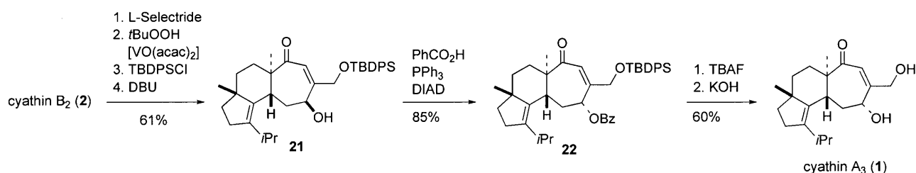
Scheme 4. Total synthesis of cyathin A 3 ( 1 ). acac = acetylacetonate, Bz = benzoyl, DBU = 1,8-diazabicyclo[5.4.0]undec-7-ene, DIAD = diisopropylazodicarboxylate, TBAF = tetra- n -butylammonium fluoride, TBDPS = tert -butyldiphenylsilyl.
