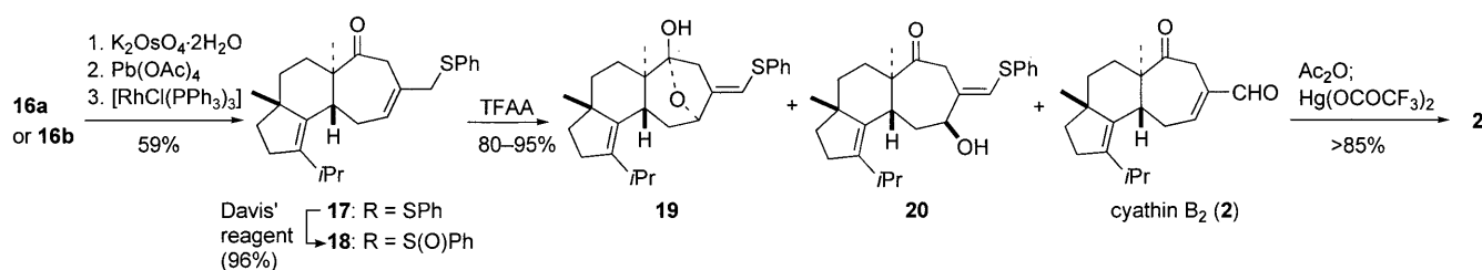
Scheme 3. Total synthesis of cyathin B 2 ( 2 ). TFAA = trifluoroacetic anhydride.
